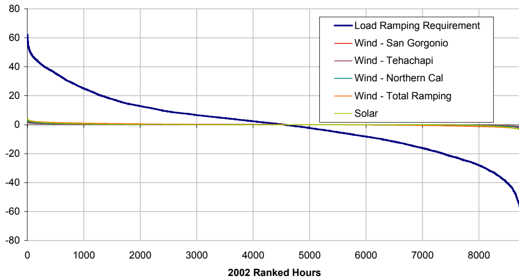
Figure 4.16. Ramping requirements for wind and solar aggregates based on hourly data; the requirements are small compared to the load ramping requirement.
