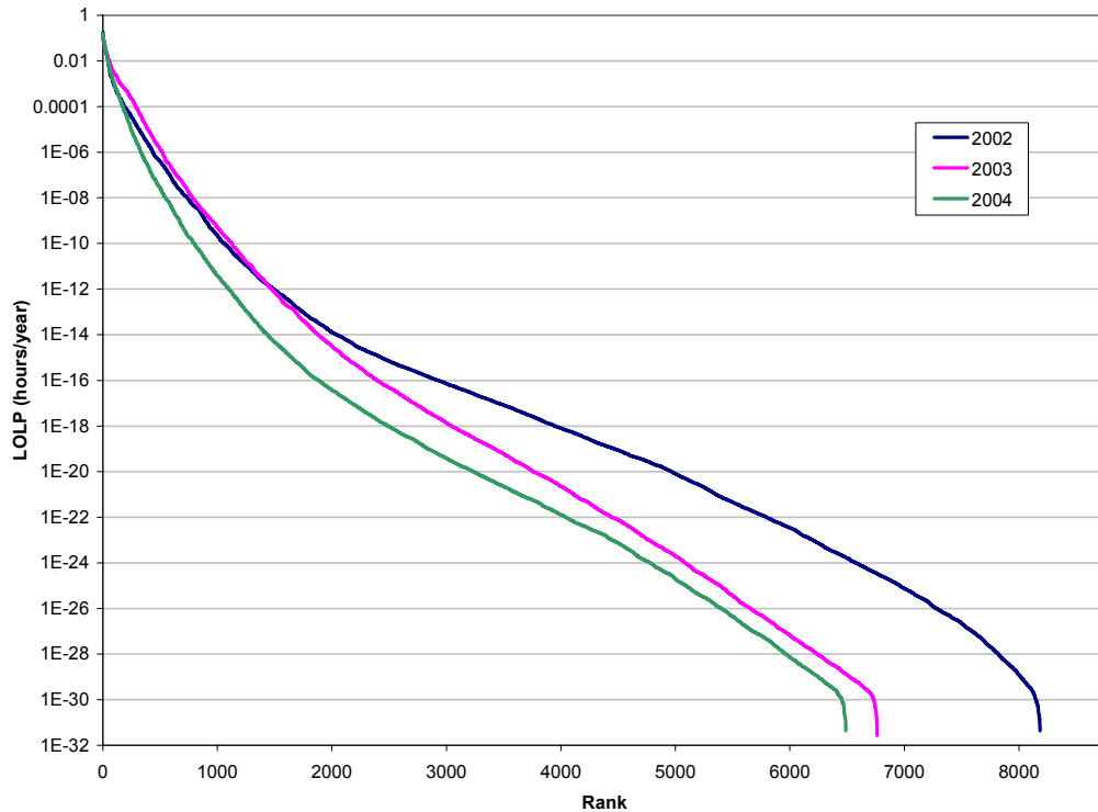
Figure 2.1. Hourly LOLP, ranked, 2002-2004.
