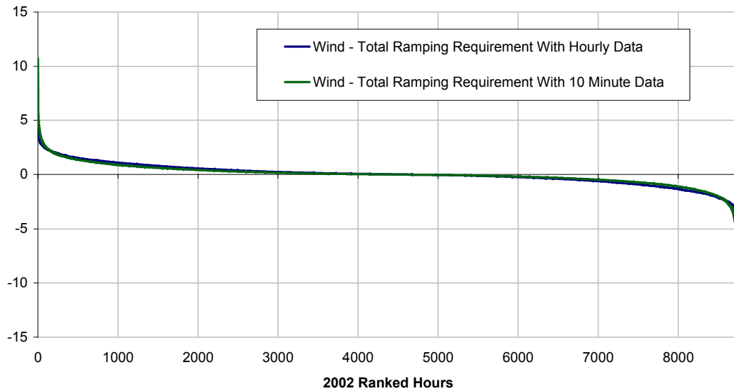
Figure 4.15. Comparison of wind ramping requirements calculated with 10 minute and hourly data.
