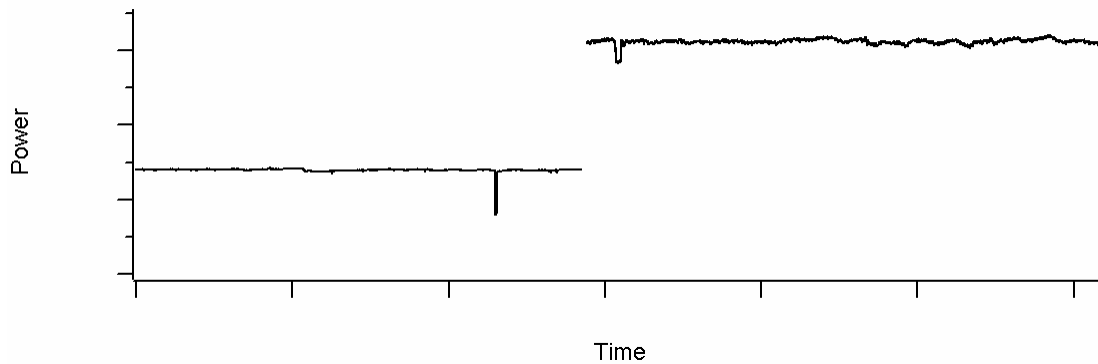
Figure 5.4. Generation of the SCE territory geothermal aggregate in the CalISO multi-year dataset. One month in spring of 2003.
